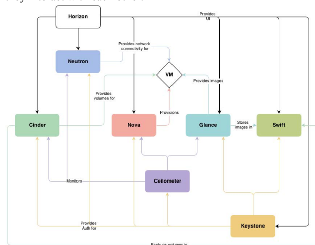
Figure 1 - Openstack conceptual architecture
